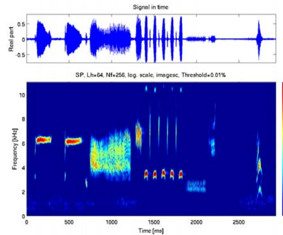
Figure 17 – Passive Sonar Spectrum
