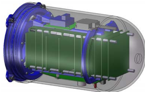
Figure 3 – Electronics Hull
