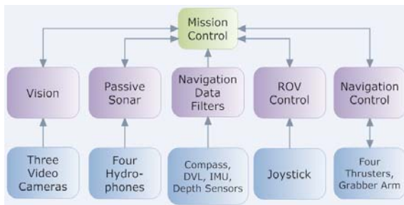
Figure 14 – Software Overview
