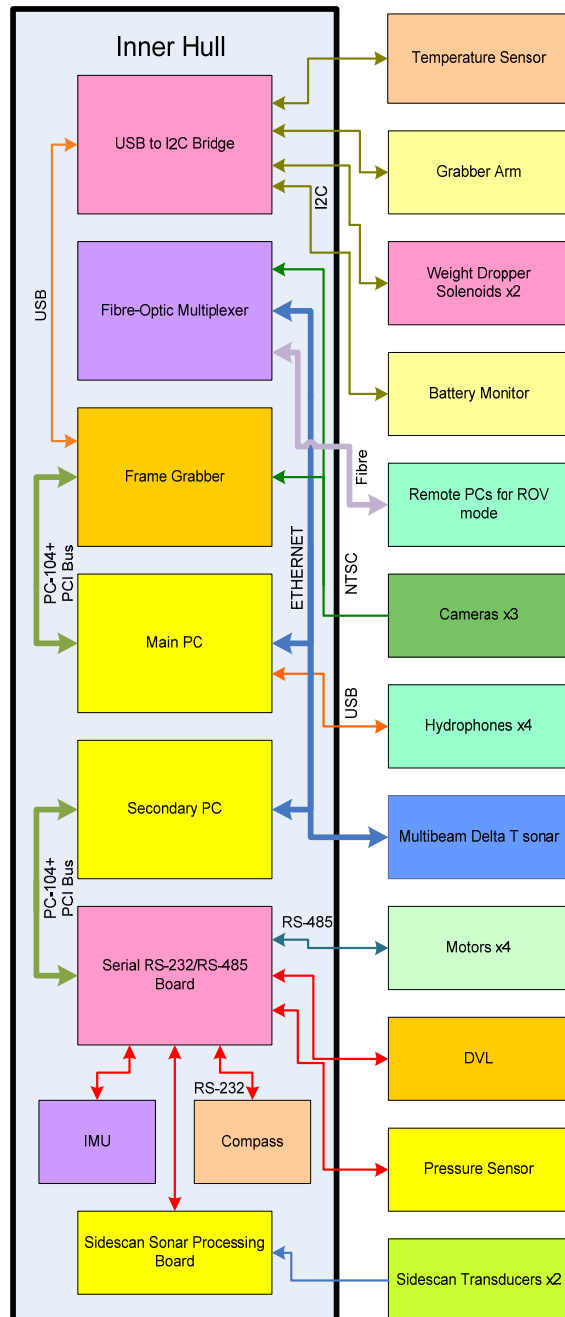
Figure 12 – Electrical Systems Schematic
