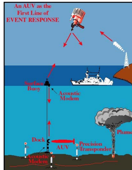
Figure 26 – AUV Rapid Response [3]
