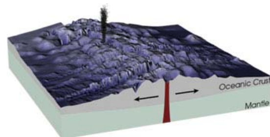
Figure 21 – Midoceanic Ridge [2]
