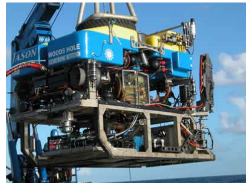
Figure 24 – The ROV Jason [3]
