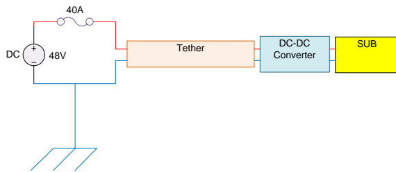
Figure 13: Grounded Fuse Safety Diagram
