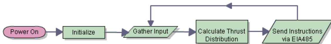
Figure 9: User interface module flow chart
