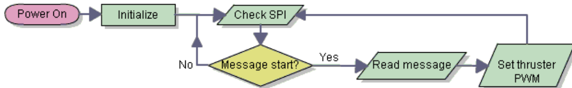
Figure 11: Thruster control module flow chart
