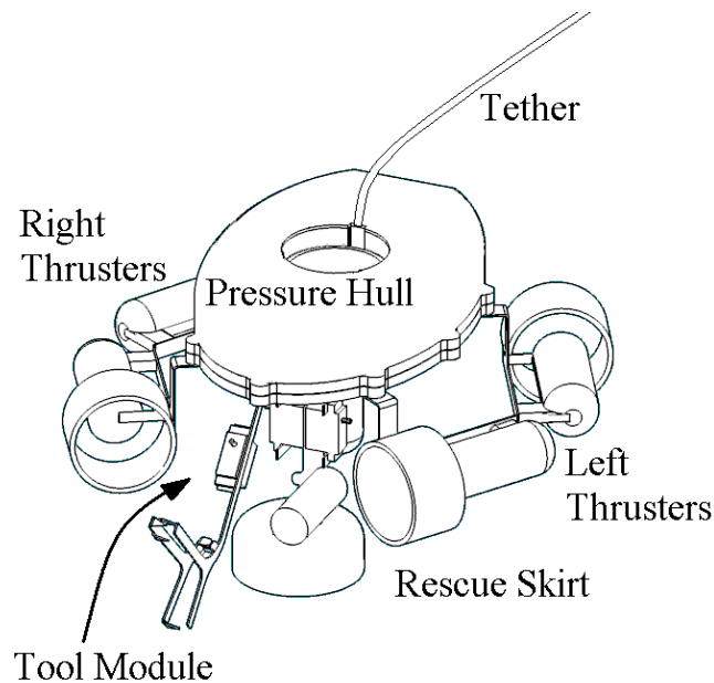
Figure 2: The ROV layout
