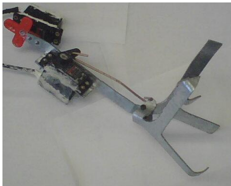
Figure 7: A tool arm with servos and linkage
