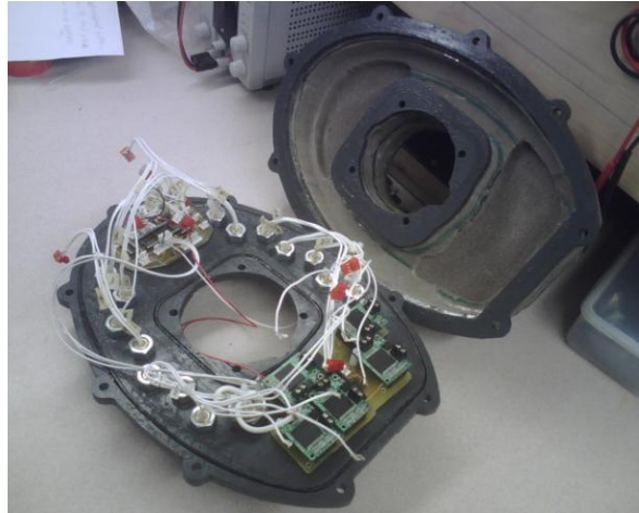
Figure 5: Pressure hull inside layout
