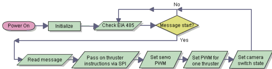
Figure 10: Tool control module flow chart
