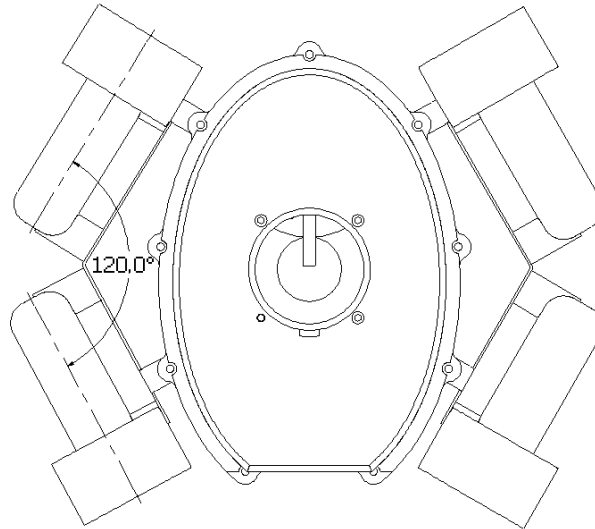
Figure 3: Thruster layout
