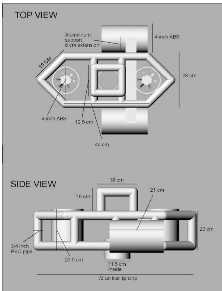
Figure 2 - Top & Side View of DAB Sans Arms/Claws
