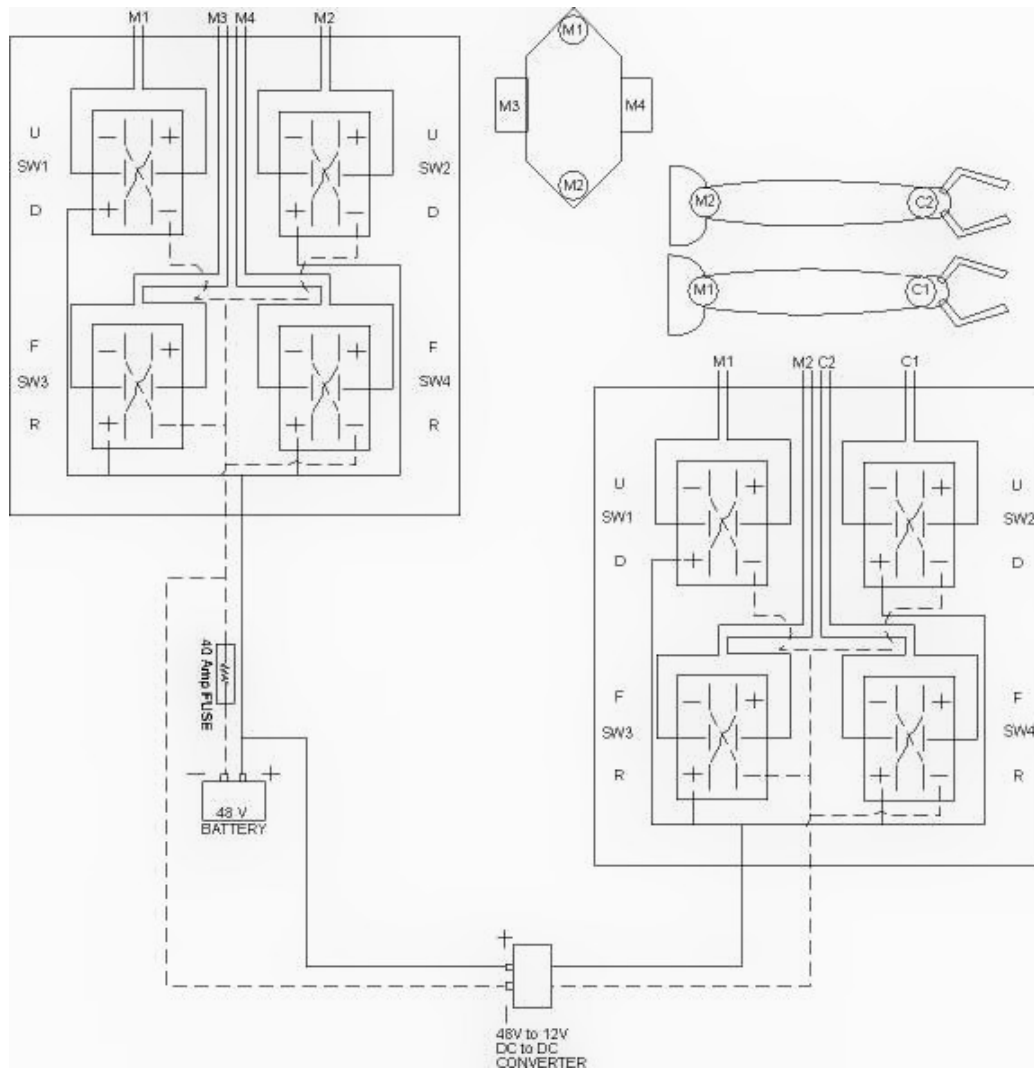
Figure 8 - DAB Electrical Schematic
