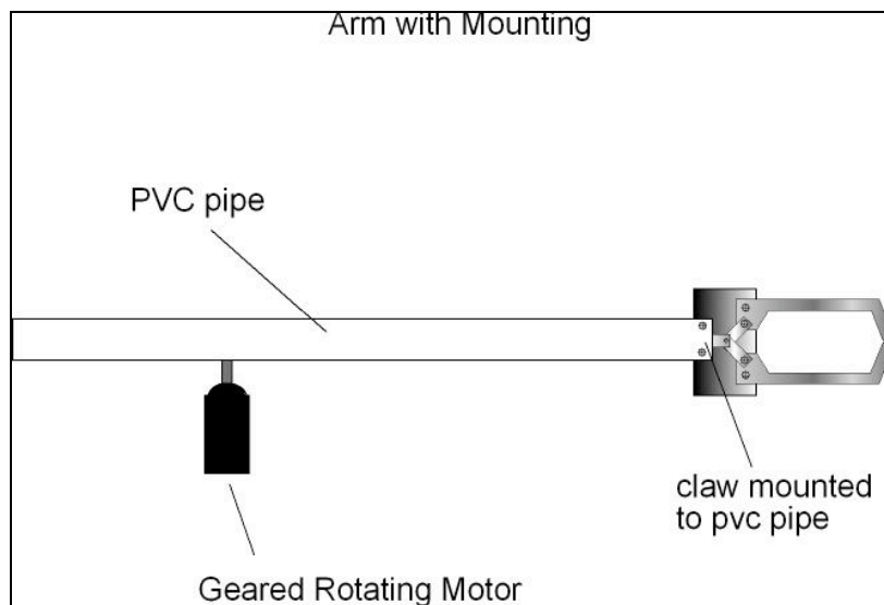
Figure 3 - DAB Arm/Claw
