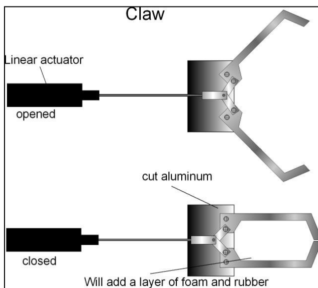
Figure 4 - DAB Claw
