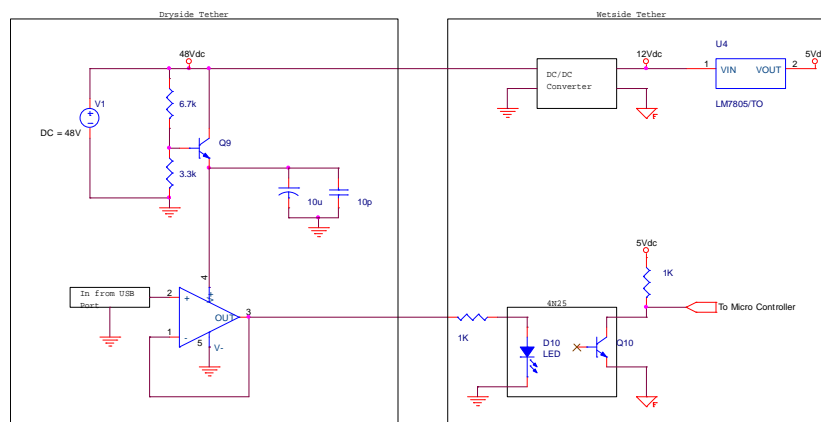
Figure 3: Tether Schematic
