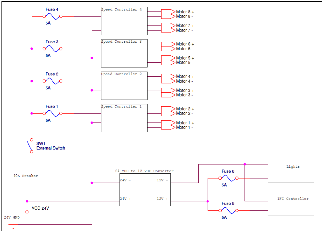
Figure 12: Electrical Circuit
