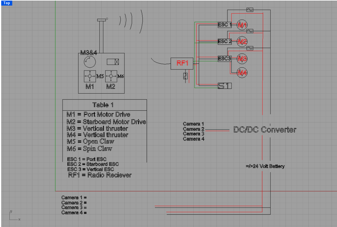
ROV Wiring Diagram
