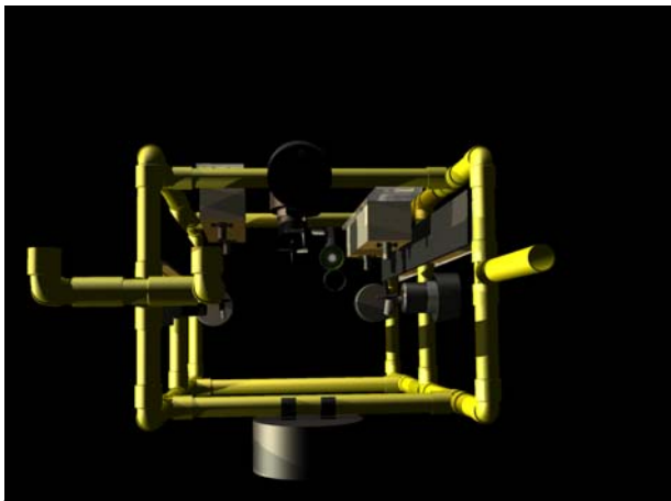
A frontal render of RUFUS MkII, done on Autodesk
