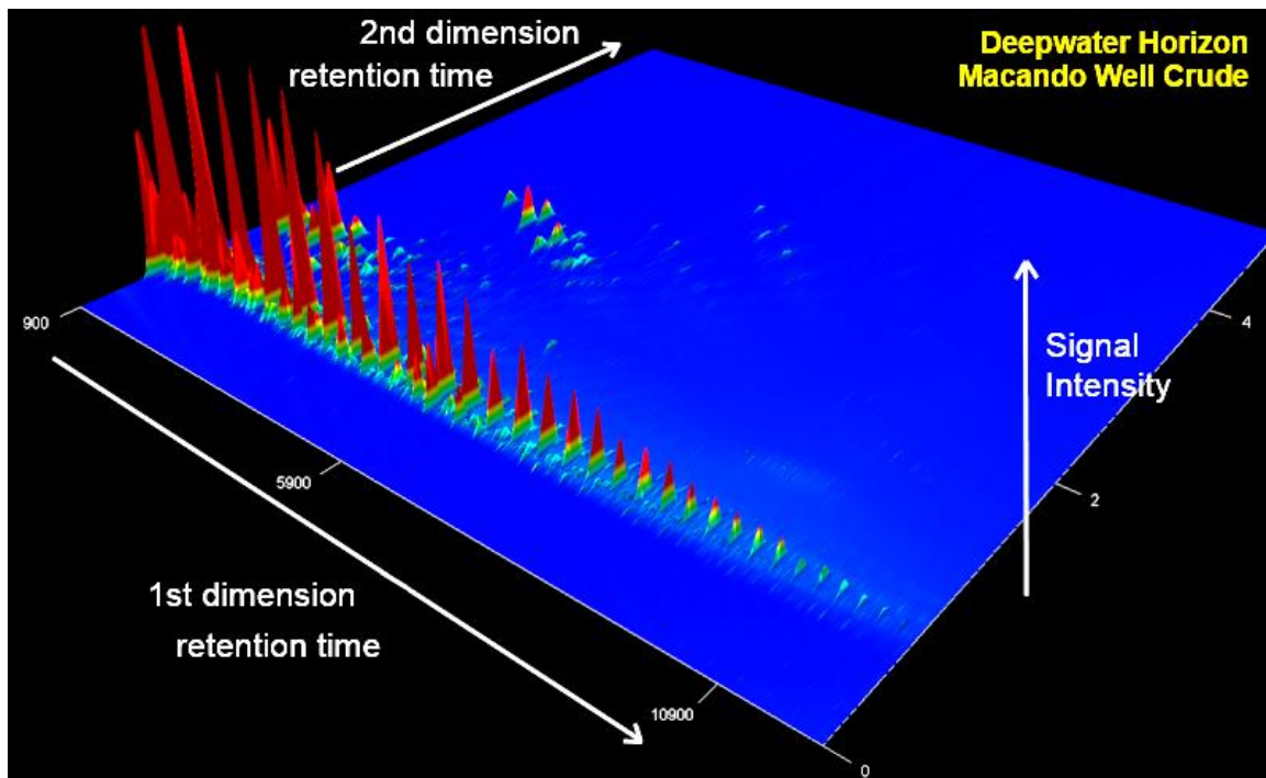
Oil sample fingerprint from the Macando well in the Gulf of Mexico.
