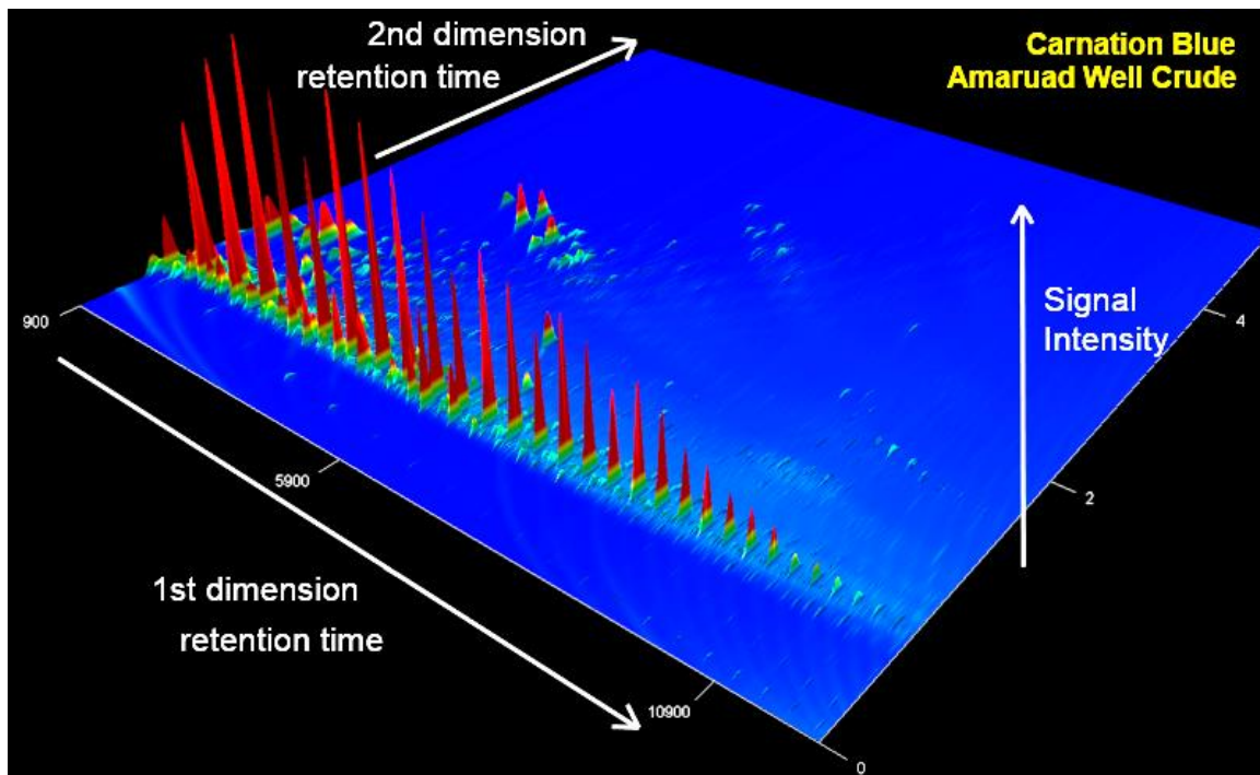
Oil sample fingerprint from the Amaruad well in the Gulf of Mexico.
