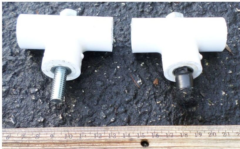
RANGER product demonstration build photo #4: Completed bolt without Velcro. Completed bolt with Velcro.
