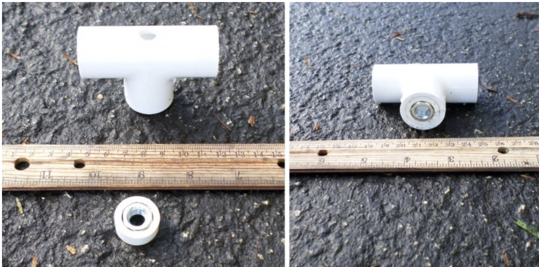
RANGER product demonstration build photo #3: PVC base of the bolt with 3/8-inch nut inserted.
