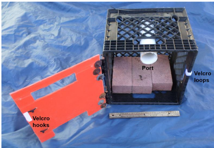
RANGER product demonstration build photo #11: The power and communications hub with the door opened, exposing the 2-inch port.
