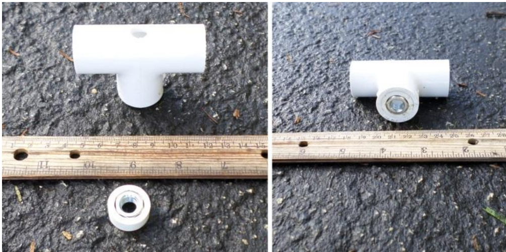
RANGER product demonstration build photo #31: PVC base of the bolt with 3/8-inch nut inserted.
