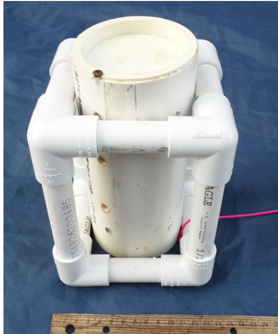
RANGER product demonstration build photo #6: The Environmental Sample Processor.
