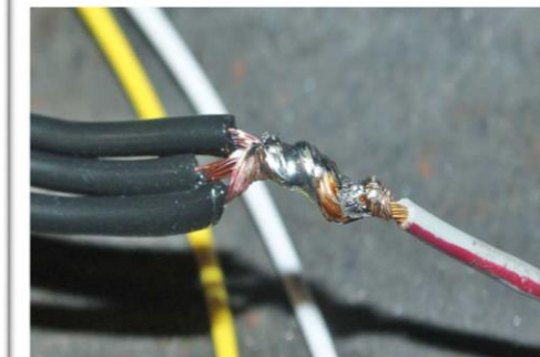
Fig 2: All electrical connections are soldered
